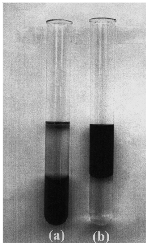
Fig. 9 Thiol-derivatisation of a hydrosol: immiscible layers of (a) a gold hydrosol (at the bottom) and a toluene solution containing dodecanethiol (on top). (b) Thiol-derivatised Au sol in the toluene layer (on top) and the clean aqueous solution at the bottom (from Sarathy et al. 35 ).
