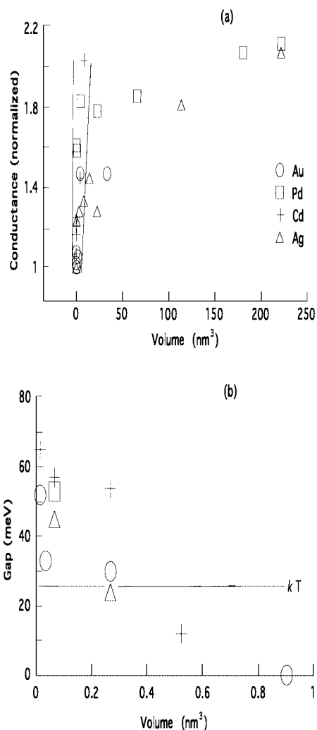
Fig. 7 Scanning tunneling spectroscopy of individual metal clusters: (a) conductance [obtained from the normalized slope of the current–voltage ( I–V ) curves] as a function of cluster volume. Above a critical volume, \sim 4 nm 3 , the slope becomes size-independent. (b) The conduction gap observed in small clusters of Au, Pd, Cd and Ag as a function of cluster volume. The volume was calculated from the cluster diameter obtained from STM (from Vinod et al. 25 ).
